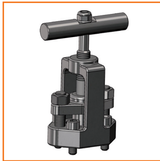
Bonnet O.S.&Y. O.S.&Y. Bonnet
